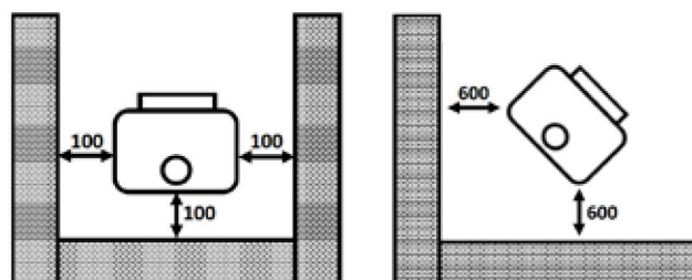
Distance to non-combustibles
