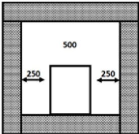
Distance to combustibles
