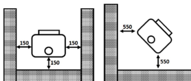
Distance to non-combustibles
