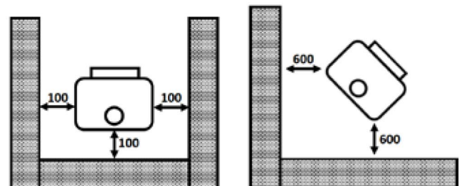
Distance to non-combustibles
